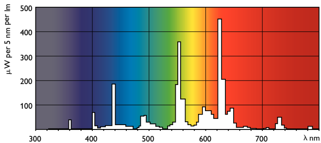
Spectral Power Distribution Colour - TL5 Essential HO 54W/830 1SL/40
