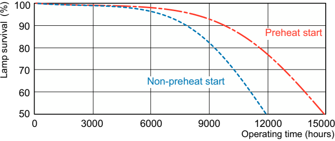
Life Expectancy Diagram - PL-T 26W/827/4P/ALTO
