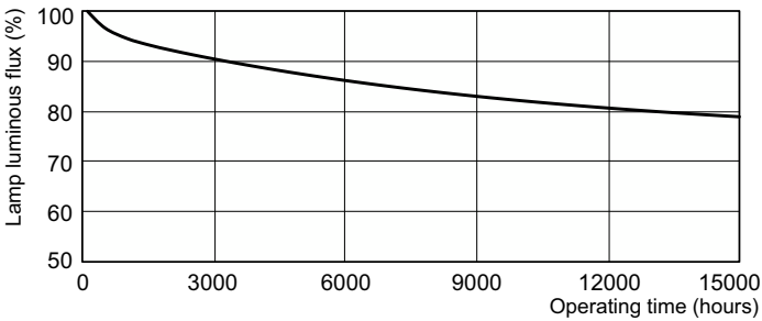
Lumen Maintenance Diagram - PL-T 26W/827/4P/ALTO
