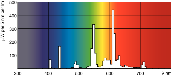
Spectral Power Distribution Colour - PL-T 26W/827/4P/ALTO
