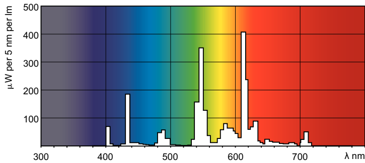
Spectral Power Distribution Colour - PL-T 26W/830/4P/ALTO
