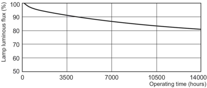
Lumen Maintenance Diagram - MASTER PL-S 7W/827/2P 1CT/5X10BOX
