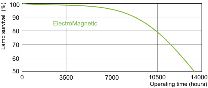
Life Expectancy Diagram - MASTER PL-S 7W/827/2P 1CT/10
