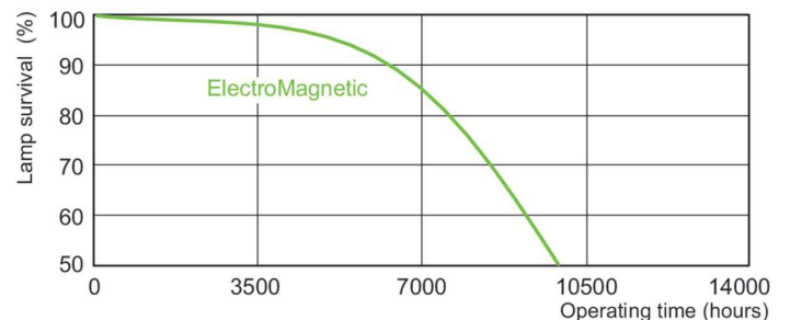
Life Expectancy Diagram - MASTER PL-S 7W/840/2P 1CT/10
