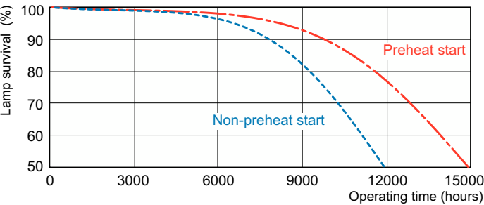
Life Expectancy Diagram - MASTER PL-S 9W/830/4P 1CT/5X10BOX
