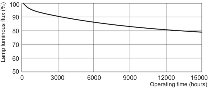
Lumen Maintenance Diagram - MASTER PL-S 9W/830/4P 1CT/5X10BOX
