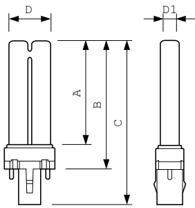
PL-S 11W/830/2P LM
