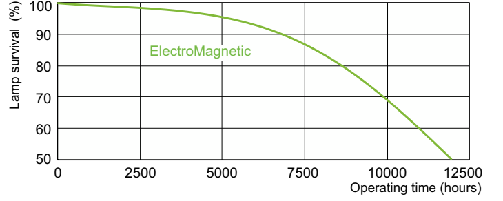
Life Expectancy Diagram - PL-Q 16W/835/2P 1CT/10BOX
