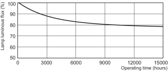
Lumen Maintenance Diagram - PL-Q 16W/835/4P 1CT/10BOX
