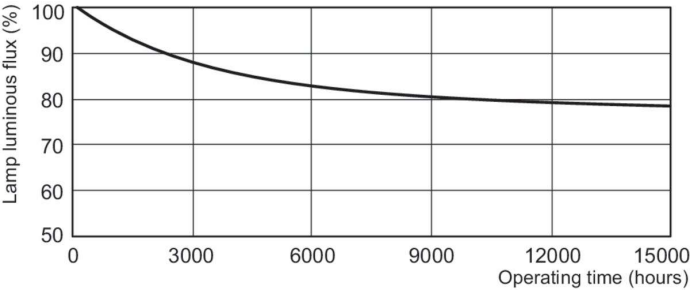
Lumen Maintenance Diagram - PL-Q 38W/835/4P 1CT/10BOX
