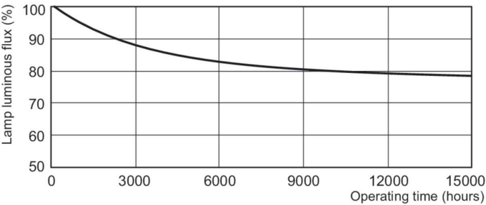
Lumen Maintenance Diagram - PL-Q 38W/840/4P 1CT/10BOX
