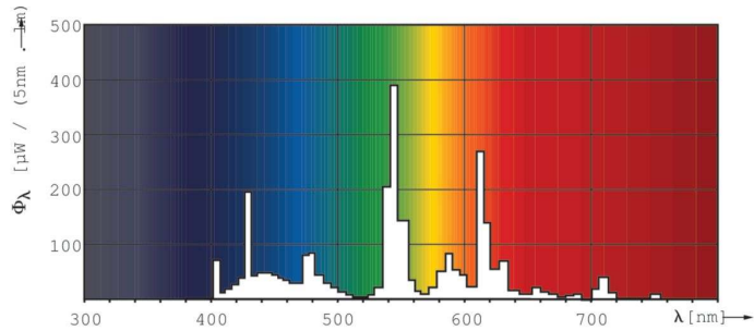
Spectral Power Distribution Colour - TL-D 18W/850 1SL/25
