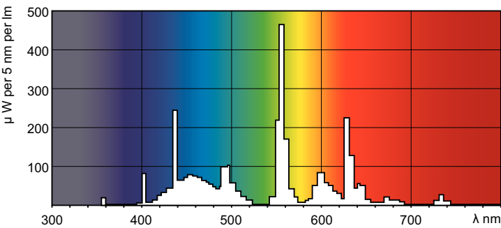
Spectral Power Distribution Colour - MASTER TL-D Xtra 58W/865 SLV
