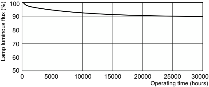
Lumen Maintenance Diagram - MASTER TL5 HO TOP 49W/840 1SL/20
