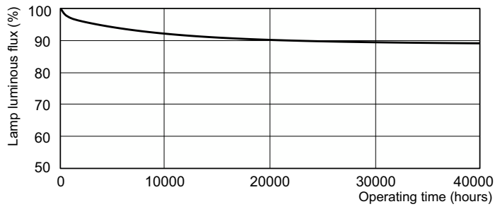
Lumen Maintenance Diagram - F54T5/835/HO/XEW/ALTO/44W
