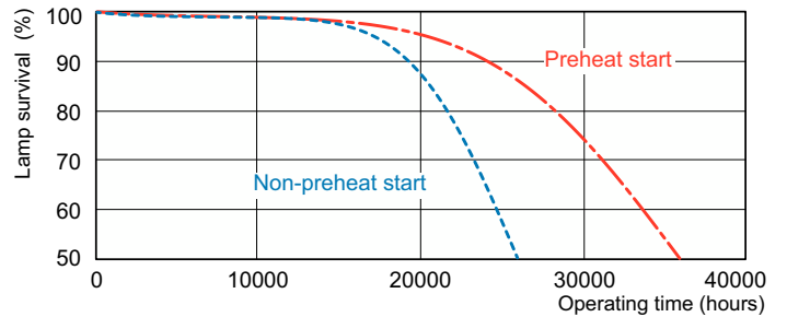
Life Expectancy Diagram - F54T5/835/HO/XEW/ALTO/44W
