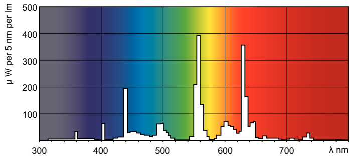
LDPO_TL5HOEPL_840-Spectral power distribution Colour
