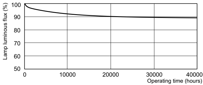
LDLM_TL5HOEPL_0001-Lumen maintenance diagram
