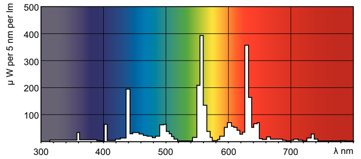
LDPO_TL5HOEPL_PLC_0001-Spectral power distribution Colour
