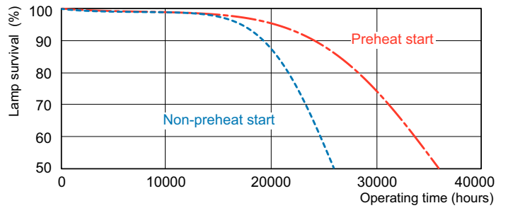
LDLE_TL5HOEPL_0002-Life expectancy diagram
