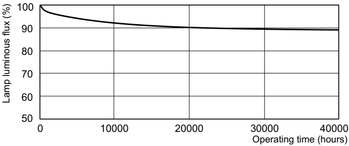
Lumen Maintenance Diagram - F54T5/850/HO/XEW/ALTO/44W
