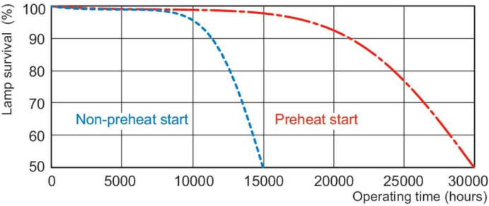
Life Expectancy Diagram - F54T5/850/HO/XEW/ALTO/44W
