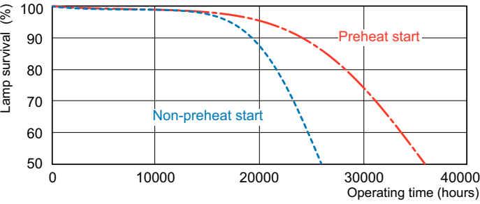
Life Expectancy Diagram - F54T5/850/HO/XEW/ALTO/44W
