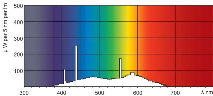
Spectral Power Distribution Colour - TL 40W/54-765 RSYL 1SL/25
