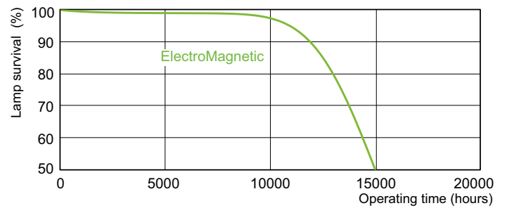
Life Expectancy Diagram - F15T8 BRIGHT WHITE/18 ALTO SL6
