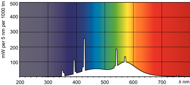
Spectral Power Distribution Colour - T10 PLUS 40W/750 1SL/25
