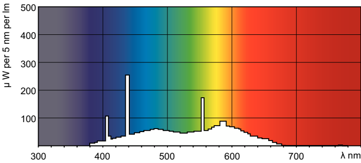
Spectral Power Distribution Colour - TL-D 58W/54 1SL/25
