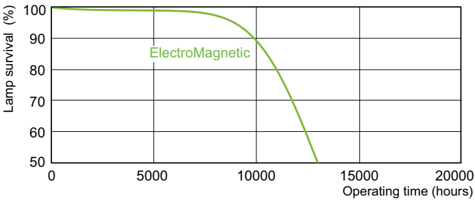
Life Expectancy Diagram - TL-D 58W/54 1SL/25
