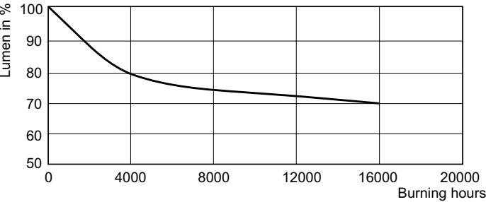
Lumen Maintenance Diagram - HPL-N 125W E27 SG 1CT/24
