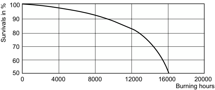
Life Expectancy Diagram - HPL-N 400W/542 E40 HG 1SL/6
