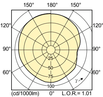
Light Distribution Diagram - MST CosmoWhite CPO-TT Xtra 315W/830 E40
