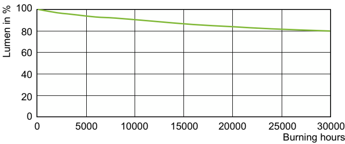
Lumen Maintenance Diagram - MST CosmoWhite CPO-TT Xtra 315W/830 E40
