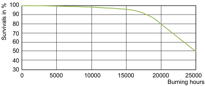
Life Expectancy Diagram - MC CDM-TC Evolution 35W/930 G8.5
