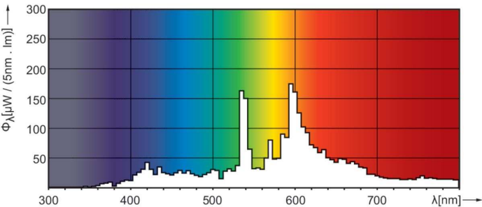
Spectral Power Distribution Colour - MASTERC CDM-R 70W/830 E26 PAR30L 40D 1CT
