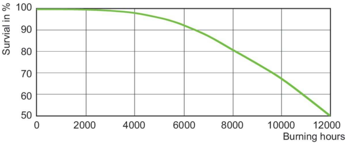
Life Expectancy Diagram - MASTERC CDM-R 70W/830 E26 PAR30L 40D 1CT
