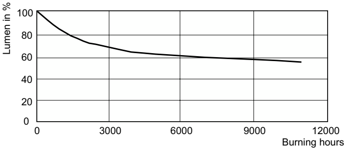
Lumen Maintenance Diagram - MASTERC CDM-R 70W/830 E26 PAR30L 40D 1CT
