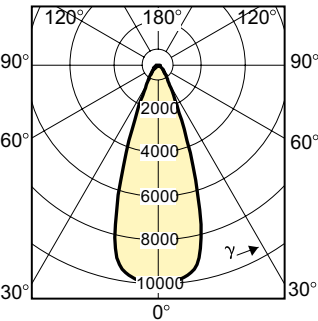
Light Distribution Diagram - MASTERC CDM-R 70W/830 E26 PAR30L 40D 1CT
