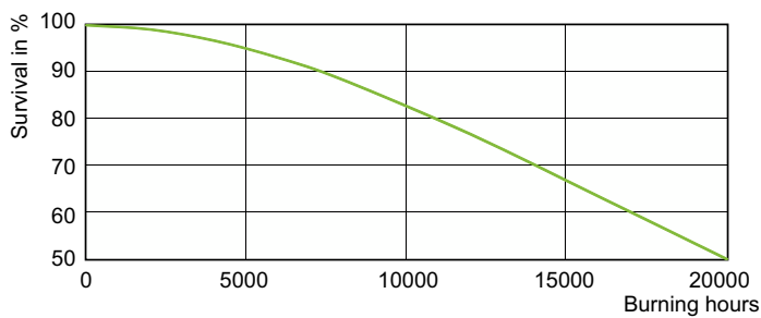
Life Expectancy Diagram - MASTER HPI Plus 250W/645 BU E40 1SL/12
