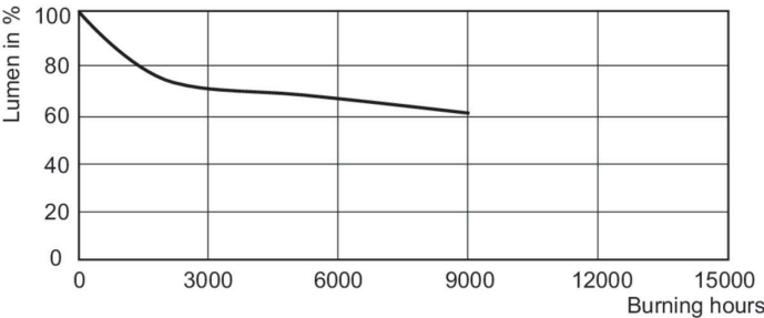
Lumen Maintenance Diagram - MHN-TD 250W/842 FC2 1CT/12
