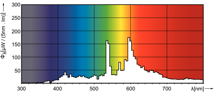
Spectral Power Distribution Colour - CDM-TD 70W/830 RX7s T6 CL
