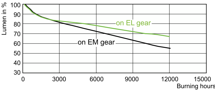
Lumen Maintenance Diagram - MASTERC CDM-T 70W/830 G12 1CT/12
