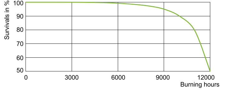
Life Expectancy Diagram - MASTER CDM-T 35W/830 G12 1CT/12
