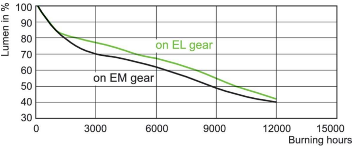
Lumen Maintenance Diagram - MASTER CDM-T 35W/830 G12 1CT/12
