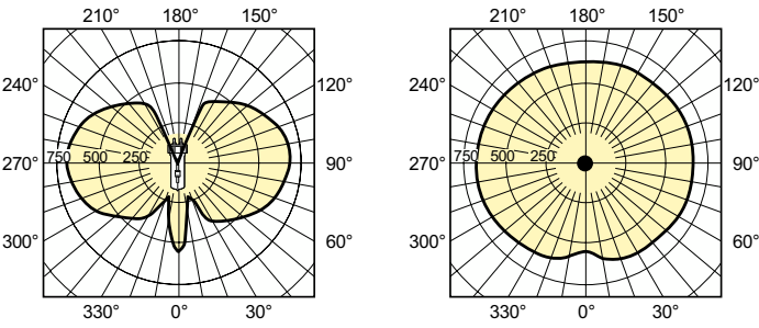
Light Distribution Diagram - CDM-T 70W/942 G12 T6 CL
