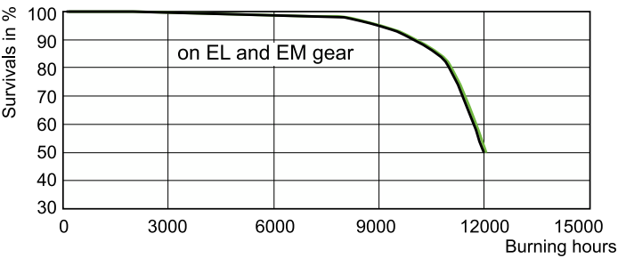
Life Expectancy Diagram - MASTER CDM-T 70W/942 G12 1CT/12
