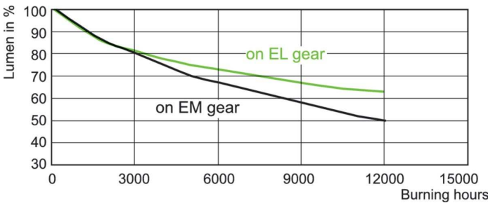
Lumen Maintenance Diagram - MASTER CDM-T 70W/942 G12 1CT/12
