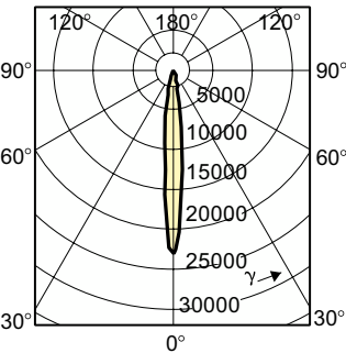
Light Distribution Diagram - MASTERC CDM-R 35W/830 E26 PAR20 10D 1CT
