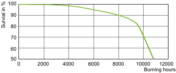
Life Expectancy Diagram - MASTERC CDM-R 35W/830 E26 PAR20 10D 1CT
