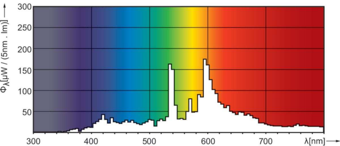
Spectral Power Distribution Colour - MASTERC CDM-R 35W/830 E26 PAR20 10D 1CT
