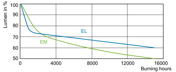
Lumen Maintenance Diagram - MASTERC CDM-TP 150W/830 PGX12-2 1CT/12
