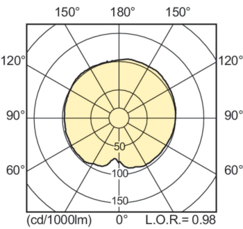
Light Distribution Diagram - CPO-TW 60W/728 White PGZ12
