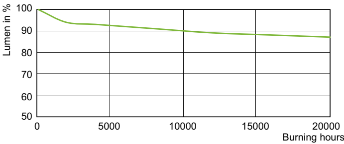
Lumen Maintenance Diagram - MST CosmoWh CPO-TW Xtra 140W/728 PGZ12
