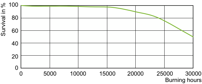
Life Expectancy Diagram - MST CosmoWh CPO-TW Xtra 140W/728 PGZ12
