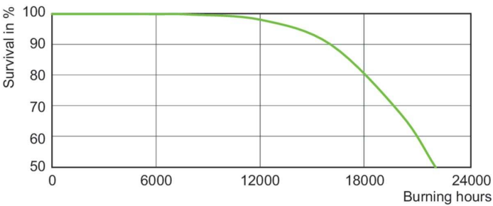
Life Expectancy Diagram - MST CosmoWh CPO-TW 60W/840 PGZ12 1CT
