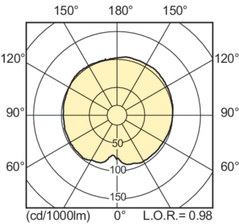
Light Distribution Diagram - MST CosmoWh CPO-TW 60W/840 PGZ12 1CT
