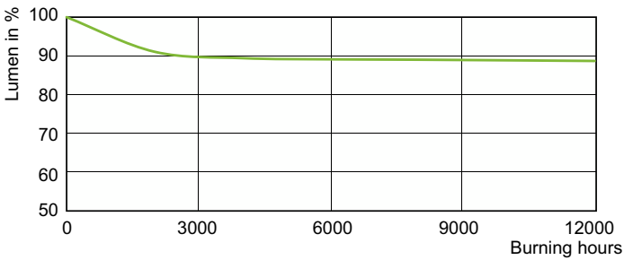
Lumen Maintenance Diagram - MST CosmoWh CPO-TW 60W/840 PGZ12 1CT
