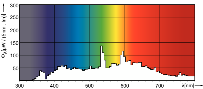
Spectral Power Distribution Colour - MASTERC CDM-R111 35W/942 GX8.5 24D 1CT
