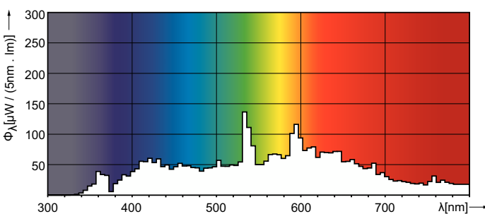
Spectral Power Distribution Colour - MASTERC CDM-R111 35W/942 GX8.5 40D 1CT/6
