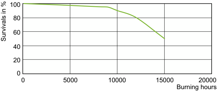
Life Expectancy Diagram - MC CDM-R Elite 70W/930 E26 PAR30L 10D
