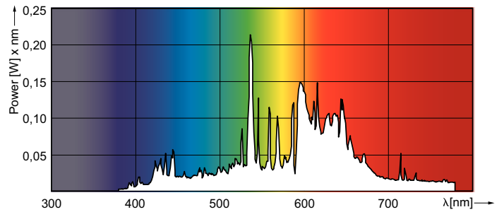
CDM-R Elite 70W /930 PAR30L
