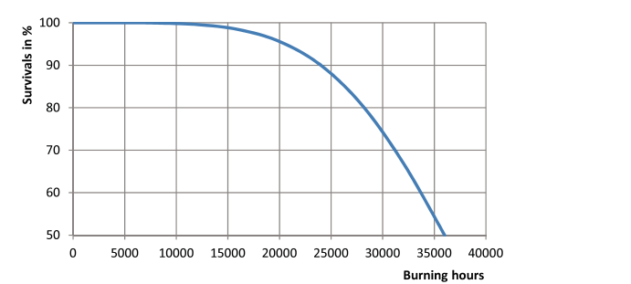
Life Expectancy Diagram - MST SON-T PIA Plus 250W E E40 1SL/12
