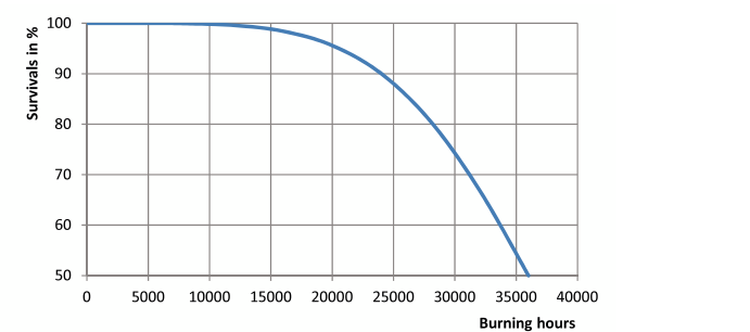
Life Expectancy Diagram - MST SON-T PIA Plus 250W E40 1SL/12
