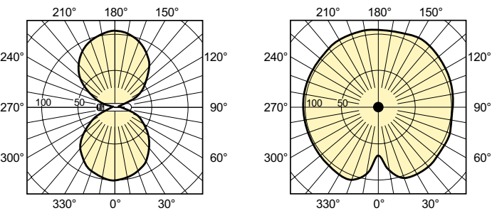
Light Distribution Diagram - SON-T PIA PLUS 250W E E40 1SL/12
