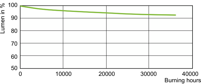
Lumen Maintenance Diagram - SON-T PIA PLUS 250W E E40 1SL/12
