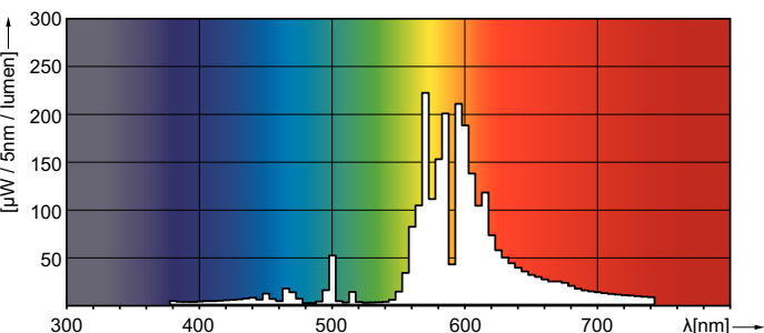
Spectral Power Distribution Colour - SON-T PIA PLUS 250W E E40 1SL/12
