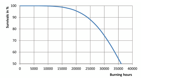
Life Expectancy Diagram - SON-T PIA PLUS 250W E E40 1SL/12
