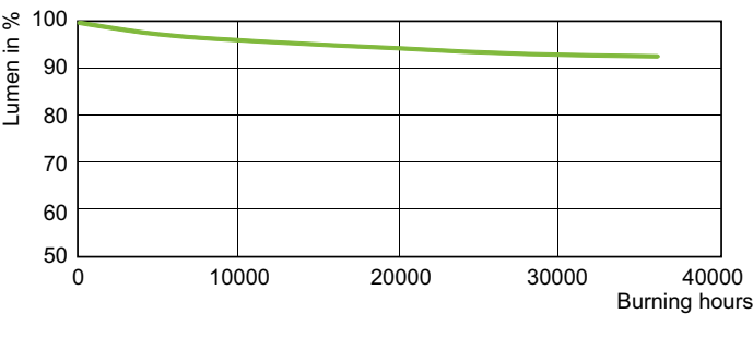
Lumen Maintenance Diagram - SON-T PIA PLUS 250W E E40 1SL/12
