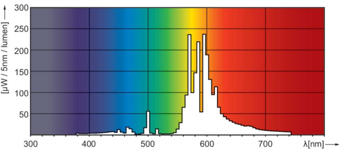
Spectral Power Distribution Colour - MST SON-T PIA Plus 400W E40 1SL/12
